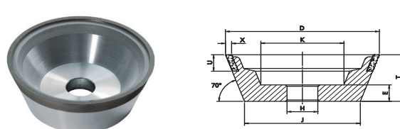
Form 11V9
