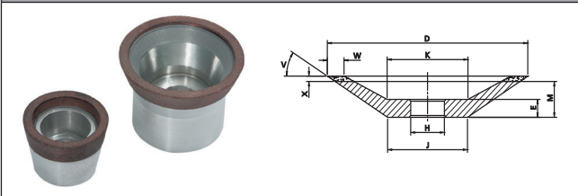
Form 12V9
