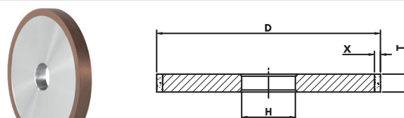
Form 1A1
