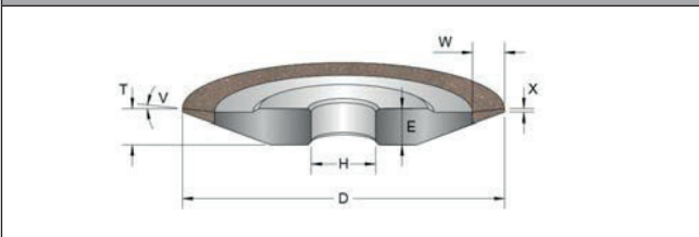
Form 6A9
